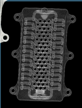
Internal Channels
