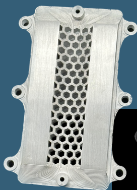
Cold Plate
