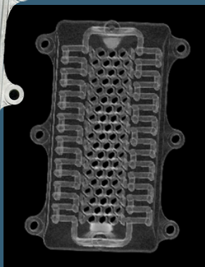
Internal Channels
